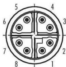
M12X
